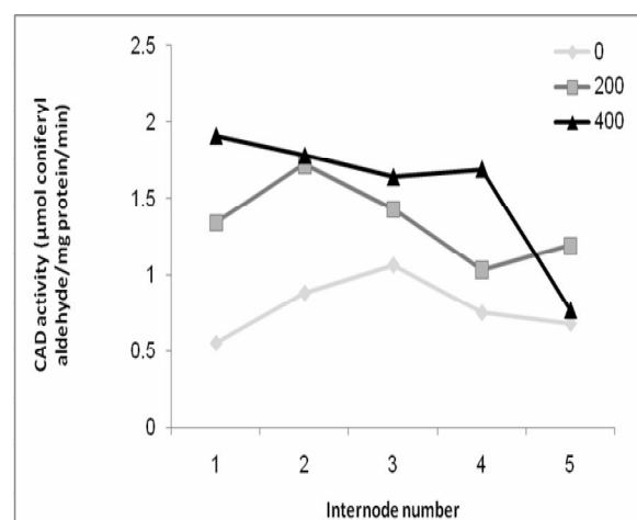
Fig. 2. Change in CAD activity under salt stress during internodal development. 1-5 Internode number from top; 1: upper and youngest internode and 5: lower internode. NaCl treatment: 0, 200 and 400 mM NaCl.
