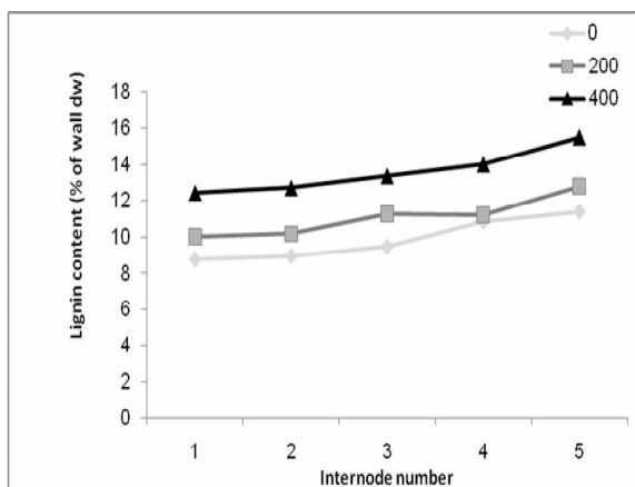
Fig. 3. Change in lignin content under salt stress during internodal development. 1-5 Internode number from top; 1: upper and youngest internode and 5: lower internode. NaCl treatment: 0, 200 and 400 mM NaCl.
