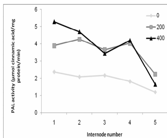
Fig. 1. Change in PAL activity under salt stress during internodal development. 1-5 Internode number from top; 1: upper and youngest internode and 5: lower internode. NaCl treatment: 0, 200 and 400 mM NaCl.
