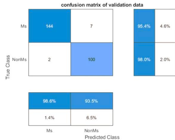
Figure 5. Confusion Matrix of the Validation Data.
