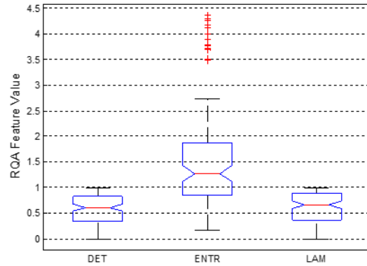
Figure 9. Boxplots of DET, ENTR, and LAM features during epileptic seizures.
