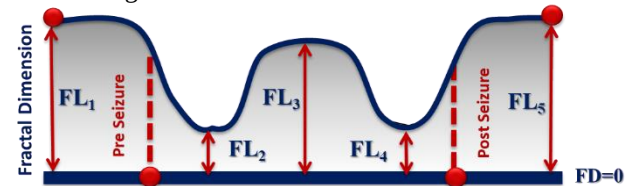
Figure 4. Identified fractal dimension pattern during epileptic seizures.
