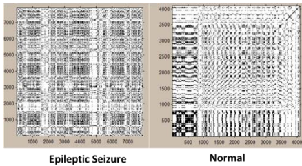
Figure 8. Recurrence plots in normal and epileptic seizure states.
