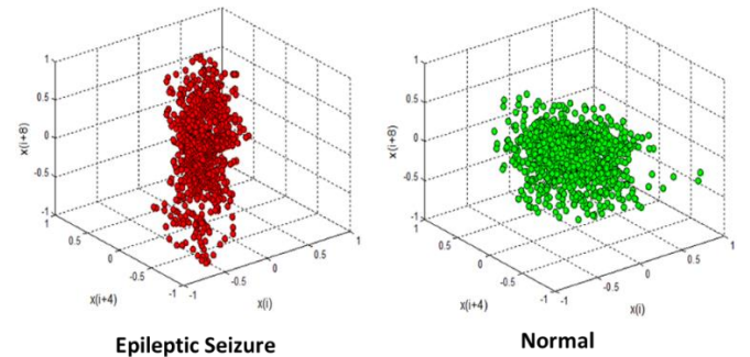
Figure 6. Phase space of EEG signals in normal and epileptic seizure states.
