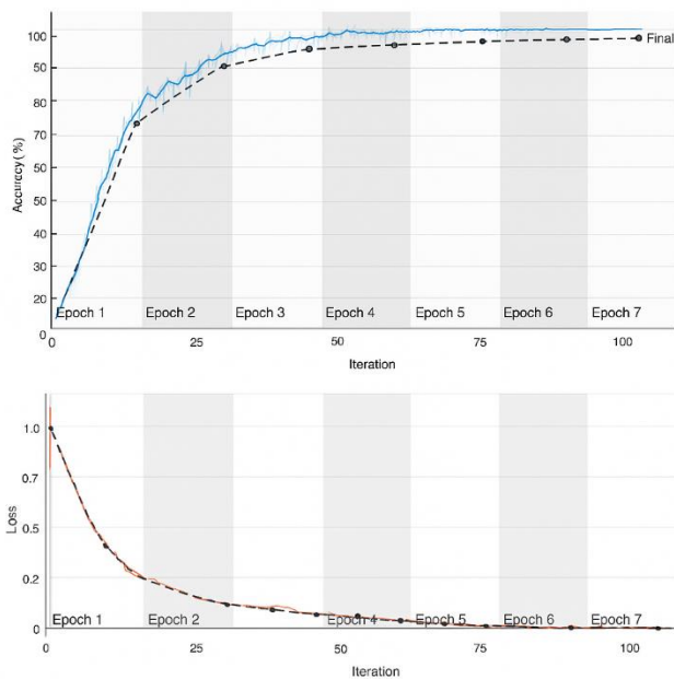
Figure 6. Training curves for the proposed CNN-LSTM model in Scenario III: up) Accuracy progression during training, down) Loss function trend illustrating model fitting improvement. Dashed lines correspond to validation dataset metrics.
