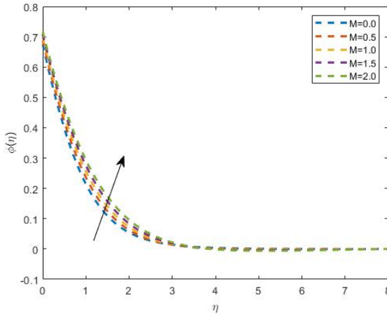
FIGURE 3. Concentration numerous values of M
