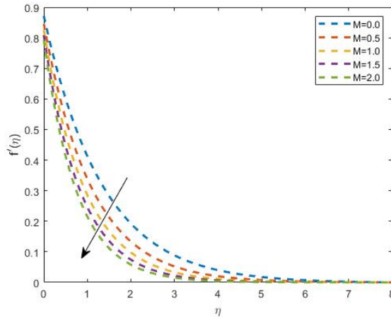
FIGURE 1. Velocity numerous values of M
