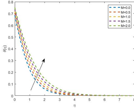
FIGURE 2. Temperature numerous values of M
