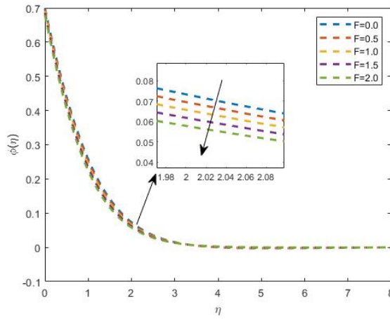
FIGURE 7. Concentration numerous values of F_r
