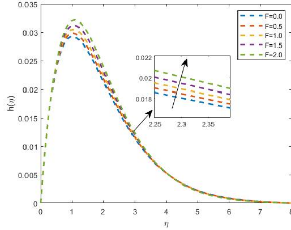
FIGURE 8. Angular numerous values of F_r
