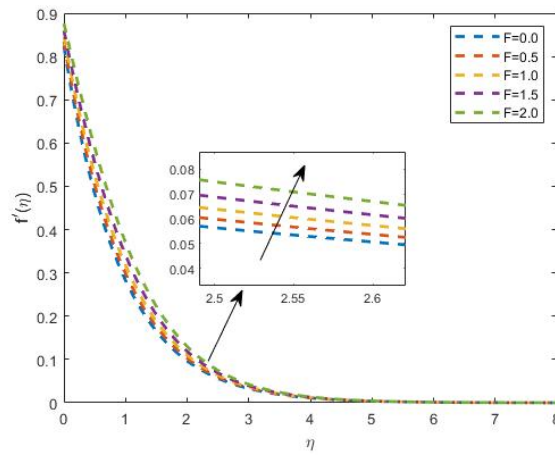
FIGURE 5. Velocity numerous values of F_r
