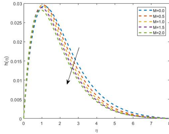
FIGURE 4. Angular numerous values of M
