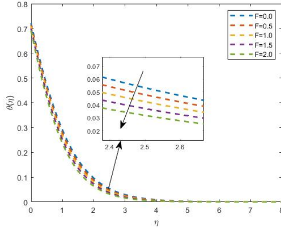
FIGURE 6. Temperature numerous values of F_r
