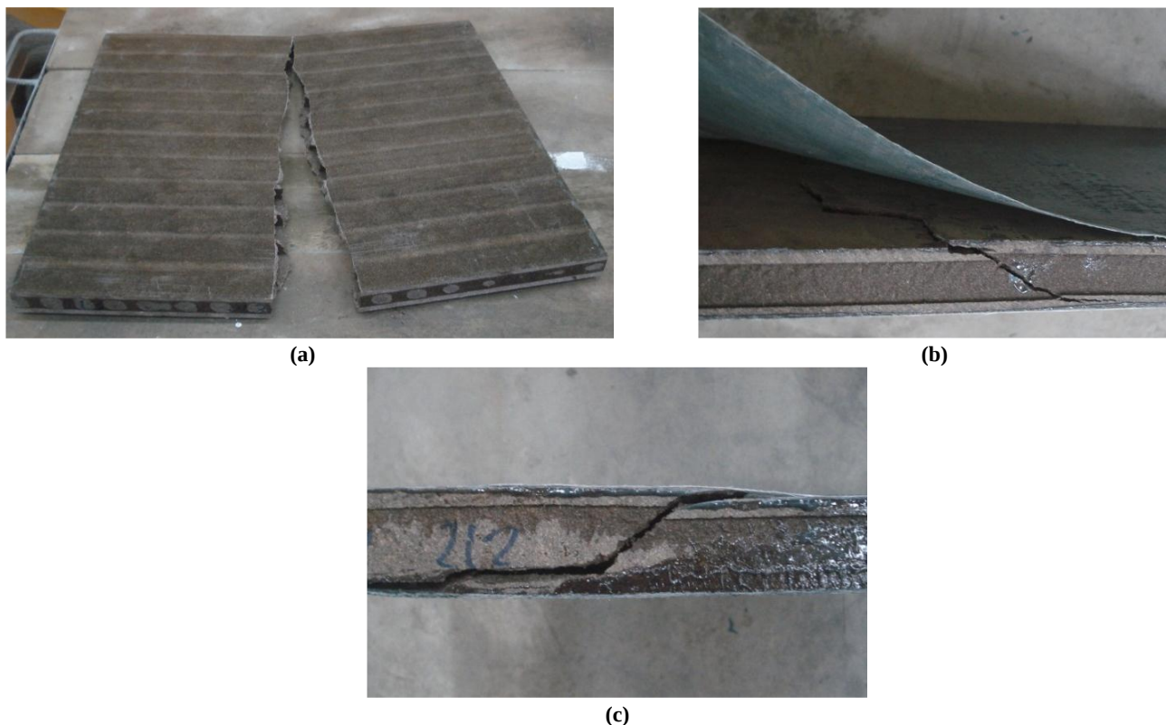
Fig. 22. Failure mode of specimens under flexural loads: (a) A0, (b) A1, and (c) A2.
