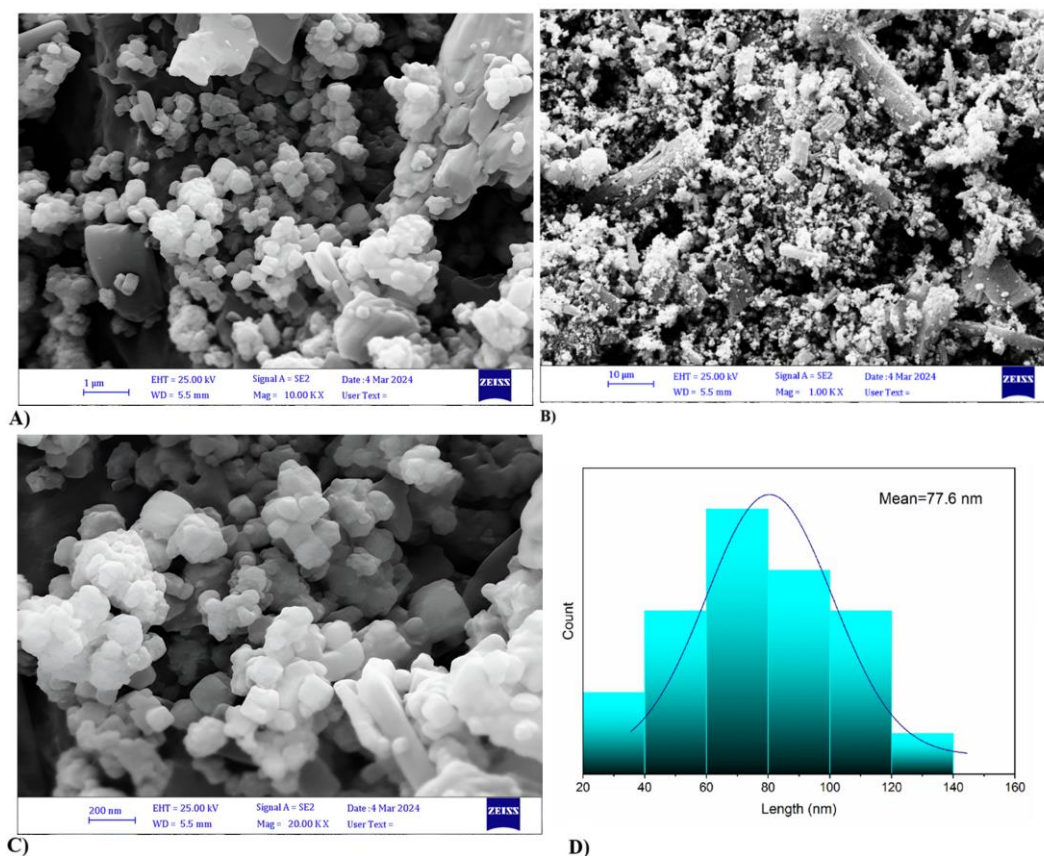
Fig. 1. FE-SEM images and size distribution of the \text{Fe}_3\text{O}_4@\text{Glu-HA-NAR} NPs. FE-SEM micrographs at different magnifications: A) 1 µm scale bar; B) 10 µm scale bar; C) 200 nm scale bar, showing spherical to cubic morphology with particle diameter ranging from 25.7 to 120 nm. D) Size distribution histogram of \text{Fe}_3\text{O}_4@\text{Glu-HA-NAR} NPs with a mean particle size of 77.6 nm.
