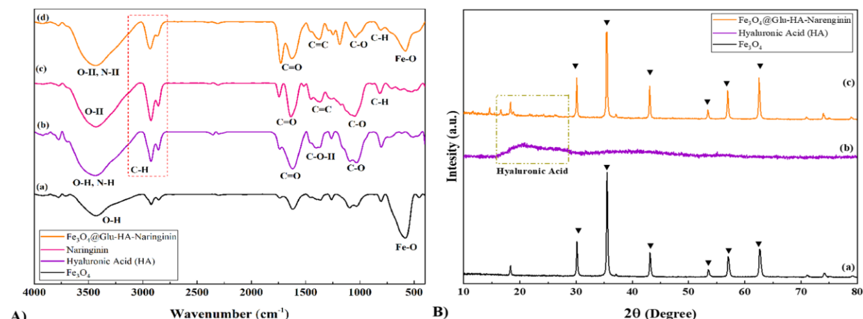
Fig. 4. FT-IR and XRD analyses of \text{Fe}_3\text{O}_4@\text{Glu-HA-NAR} NPs and their constituent materials: A) FT-IR spectra of (a) \text{Fe}_3\text{O}_4 , (b) Hyaluronic acid (HA), (c) NAR, and (d) \text{Fe}_3\text{O}_4@\text{Glu-HA-NAR} NPs. The characteristic absorption peaks of Fe-O bond ( 583\text{ cm}^{-1} ), C=C ( 801\text{ cm}^{-1} ), C-O ( 1185\text{ cm}^{-1} ), C-H ( 1376\text{ cm}^{-1} ), C=O ( 1631\text{ cm}^{-1} ), C-H ( 2930\text{ cm}^{-1} ), and O-H/N-H bonds ( 3450 and 3770\text{ cm}^{-1} ) in the composite spectrum confirm the successful incorporation of all constituent materials. B) XRD patterns of (a) \text{Fe}_3\text{O}_4 , (b) Hyaluronic acid (HA), and (c) \text{Fe}_3\text{O}_4@\text{Glu-HA-NAR} NPs. The characteristic diffraction peaks of \text{Fe}_3\text{O}_4 at 2\theta = 30.09^\circ, 35.58^\circ, 43.09^\circ, 49.53^\circ, 56.96^\circ , and 62.52^\circ , along with the amorphous broad peaks between 10\text{-}30^\circ attributed to HA, confirm the successful synthesis of the nanocomposite structure.
